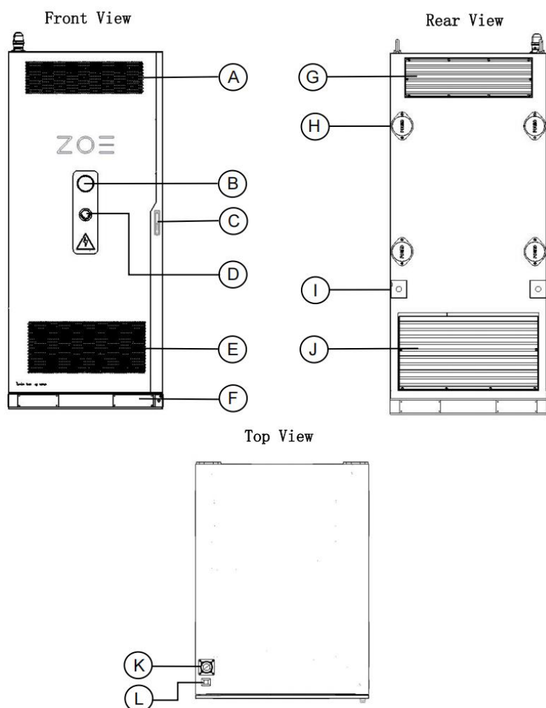
Figure 2.1 Product exterior schematic
