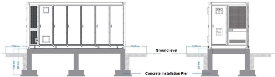
Figure 3-3 Schematic Figure of Single Container Installation Foundation
