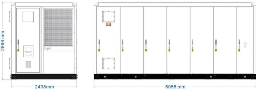
Figure 2-4 Battery Container Dimensions Figure
