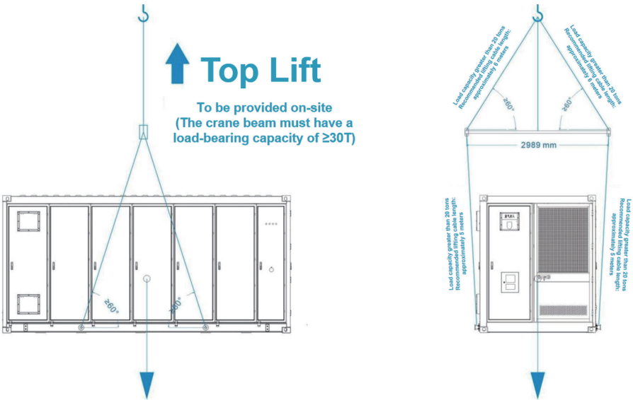
Figure 3-7 Lifting Sling Connection Figure
