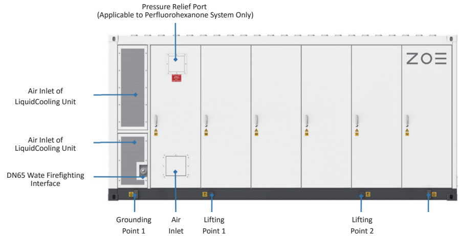
Figure 2-2 Front View of Battery Container
