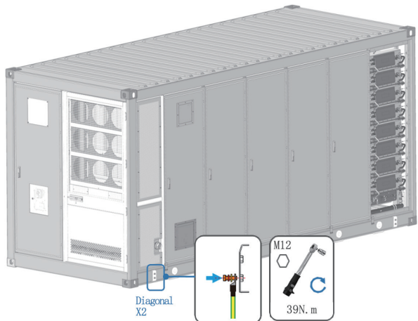
Figure 4-1 Grounding Connections for the Container
